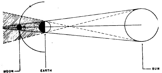
Fig. 4—Showing an eclipse of the moon.
