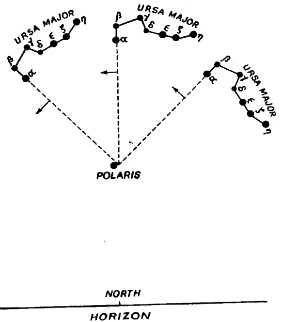
Fig. 8—Showing the positions of Ursa Major ( Saptarshi ) at interval of 3 hours.
